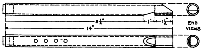
STOCK 1 BAMBOO ABOUT 14" LONG - 2 CORKS FIG. 2
